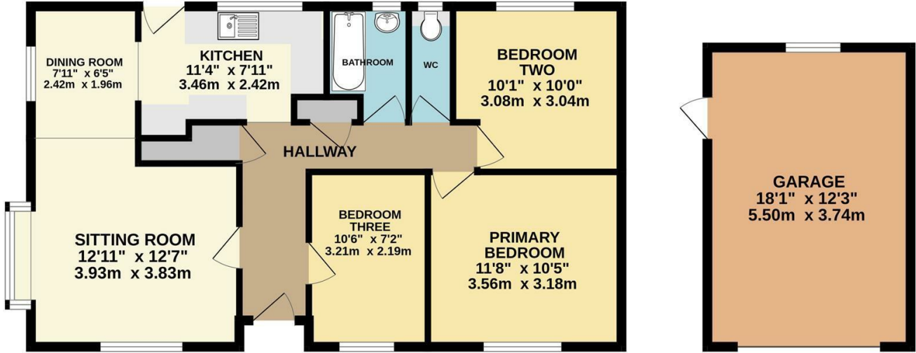
GROUND FLOOR 951 sq.ft. (88.4 sq.m.) approx.
